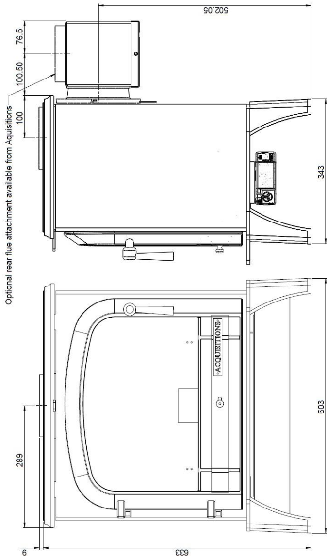
Fig 1 –Bloomsbury Gas Stove Dimensions
